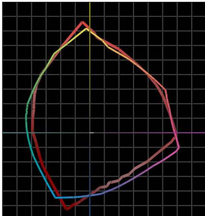
Epson SureColor SC-T3200 colour gamut on plain paper in Speed settings (red) versus Canon imagePROGRAF iPF670 colour gamut (shown chromatically) on plain paper in Fast settings.
